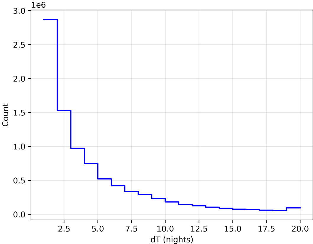
too_elab_r16_d2_gz_v3.4_10yrs All sky all bands: DeltaNight Histogram
