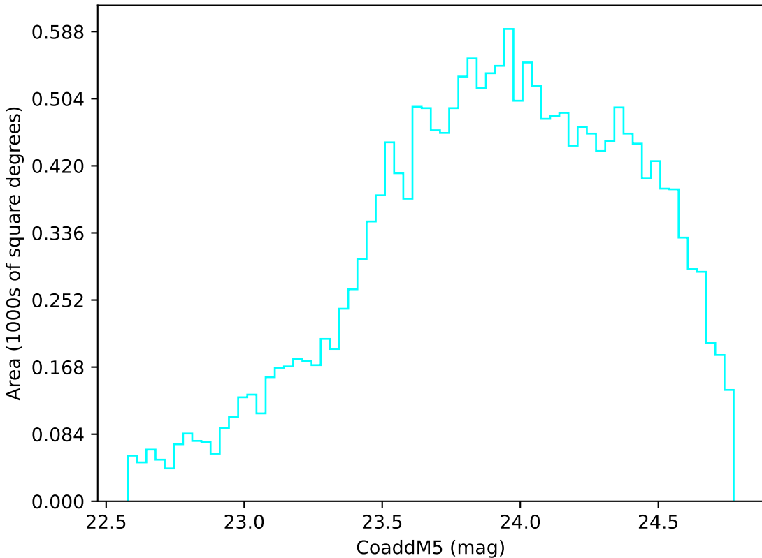
too_elab_r16_d2_gz_v3.4_10yrs Yr 3-4 u band: CoaddM5
