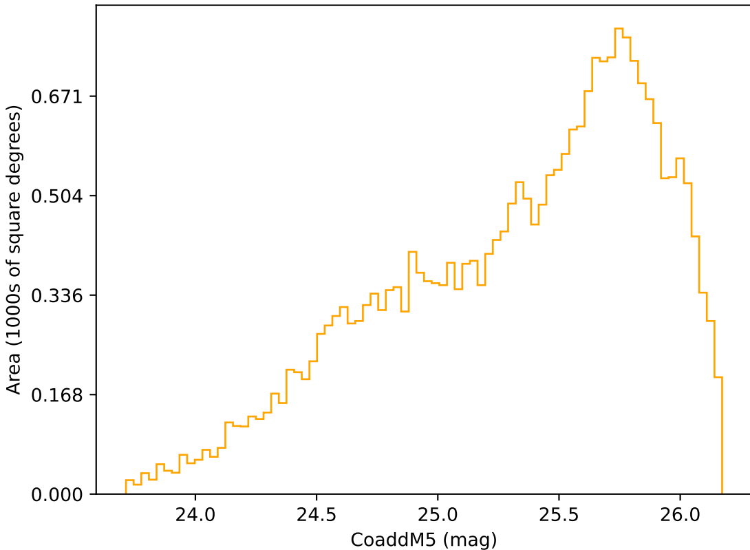
too_elab_r16_d2_gz_v3.4_10yrs Yr 3-4 r band: CoaddM5
