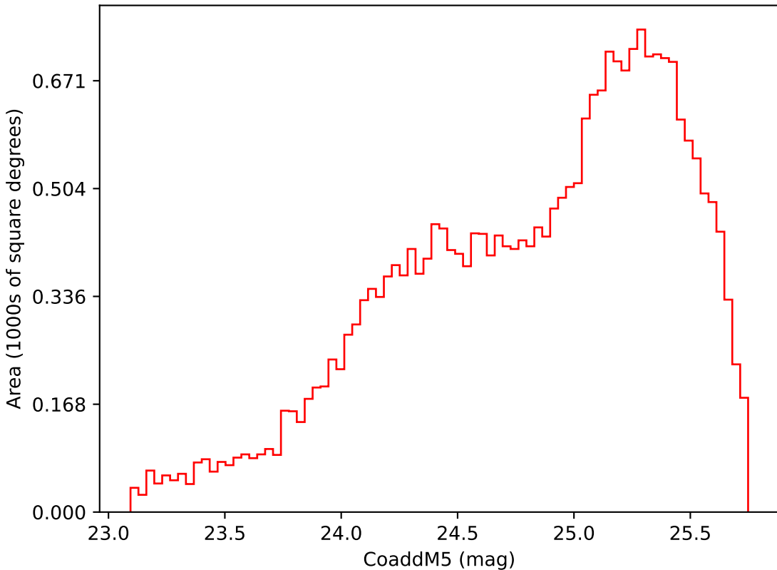
too_elab_r16_d2_gz_v3.4_10yrs Yr 3-4 i band: CoaddM5
