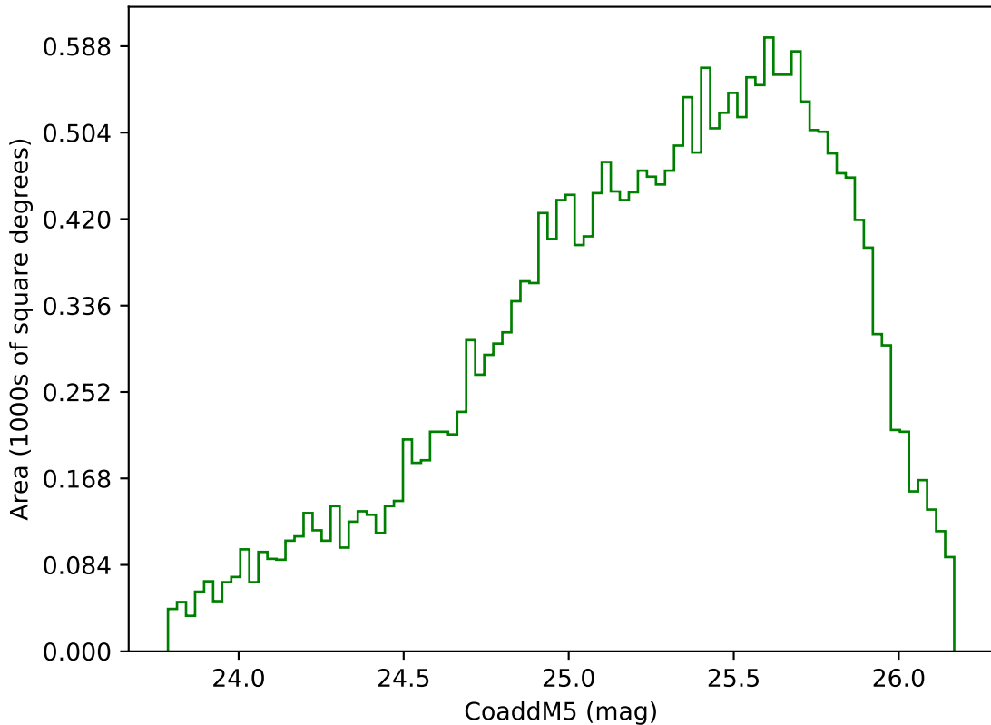
too_elab_r16_d2_gz_v3.4_10yrs Yr 3-4 g band: CoaddM5
