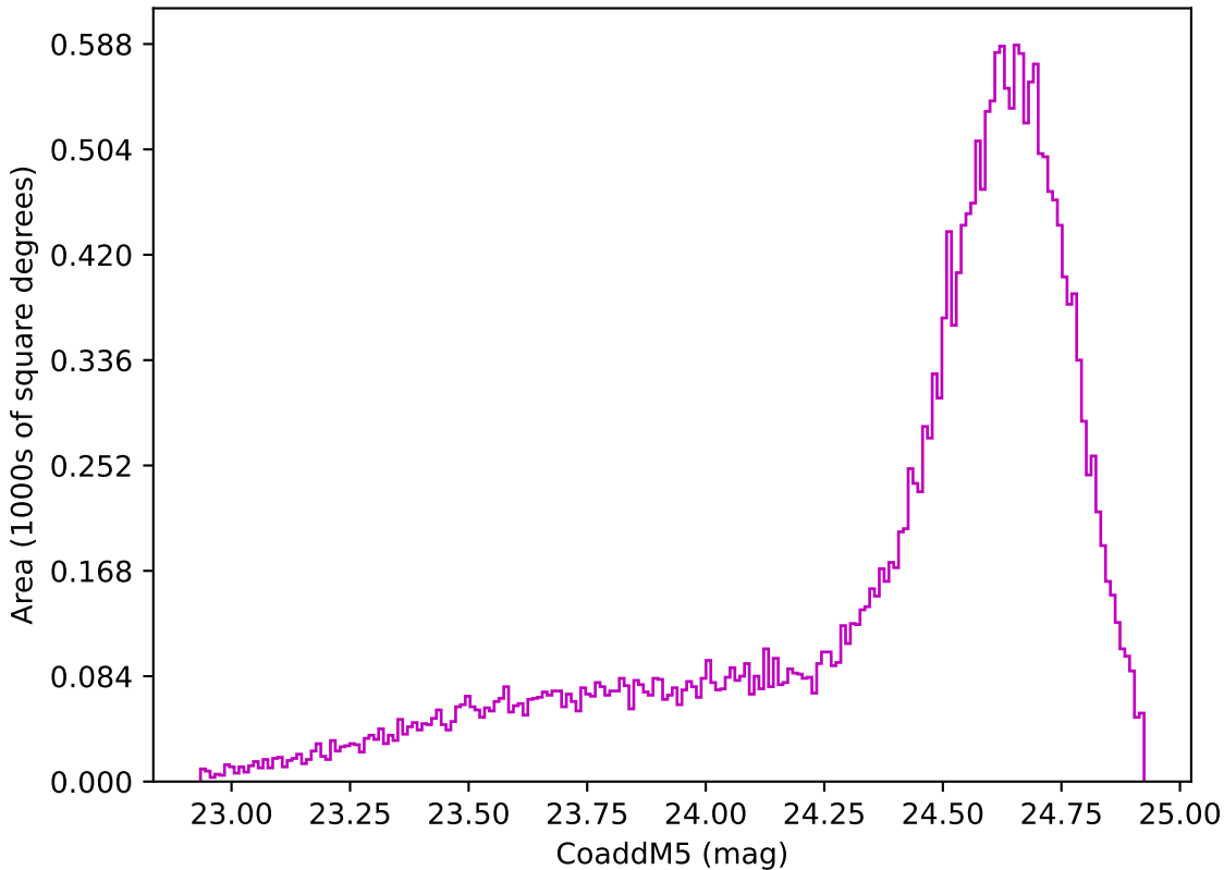
too_elab_r16_d2_gz_v3.4_10yrs Yr 1 z band: CoaddM5
