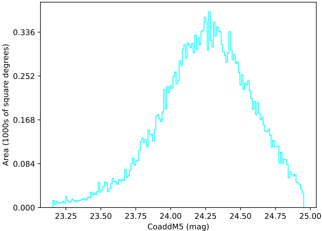
too_elab_r16_d2_gz_v3.4_10yrs Yr 1 u band: CoaddM5
