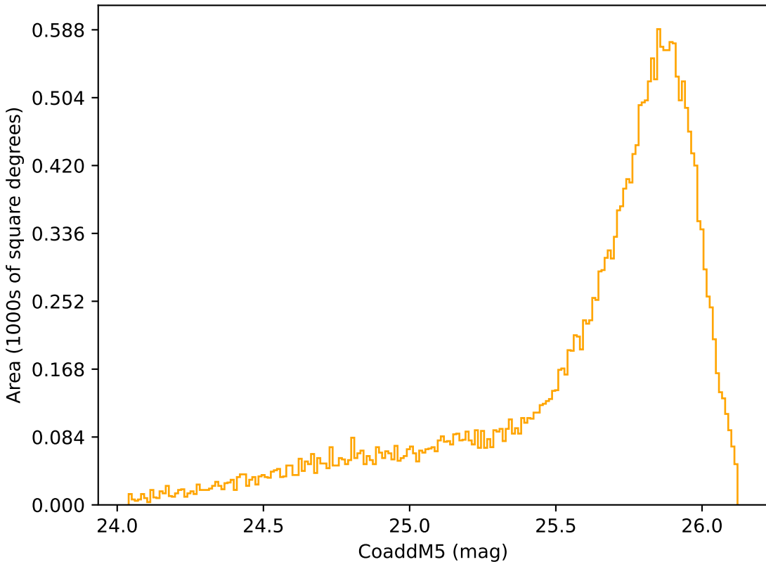
too_elab_r16_d2_gz_v3.4_10yrs Yr 1 r band: CoaddM5
