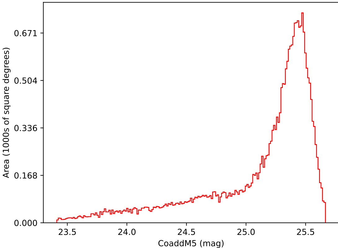
too_elab_r16_d2_gz_v3.4_10yrs Yr 1 i band: CoaddM5
