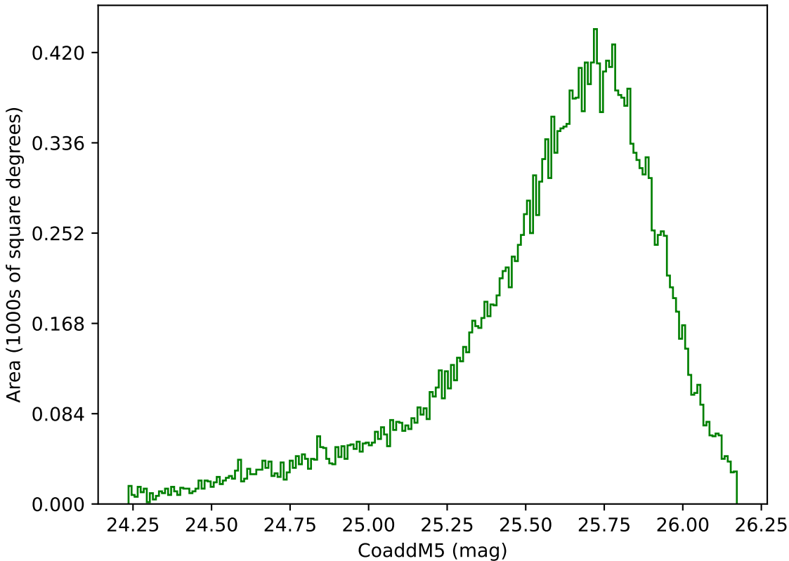
too_elab_r16_d2_gz_v3.4_10yrs Yr 1 g band: CoaddM5
