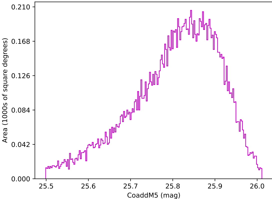
too_elab_r16_d2_gz_v3.4_10yrs WFD z band: CoaddM5
