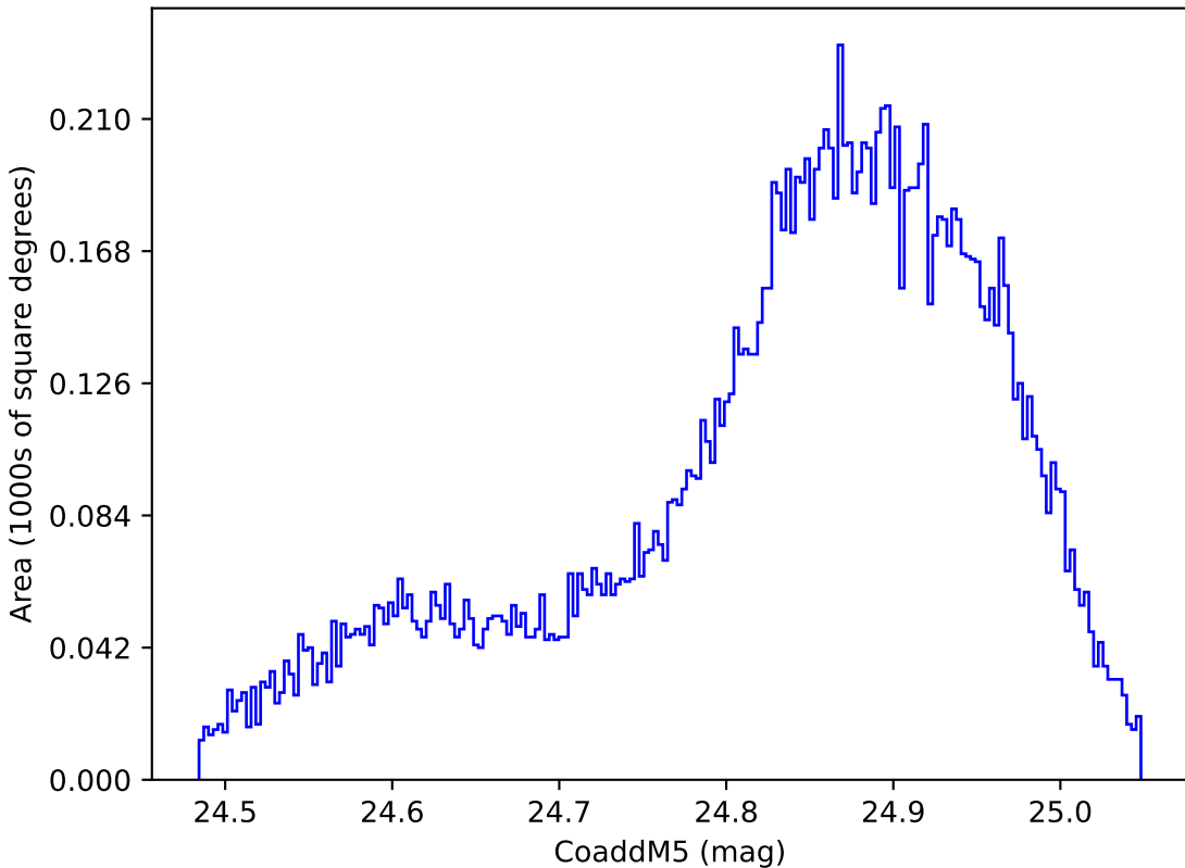
too_elab_r16_d2_gz_v3.4_10yrs WFD y band: CoaddM5
