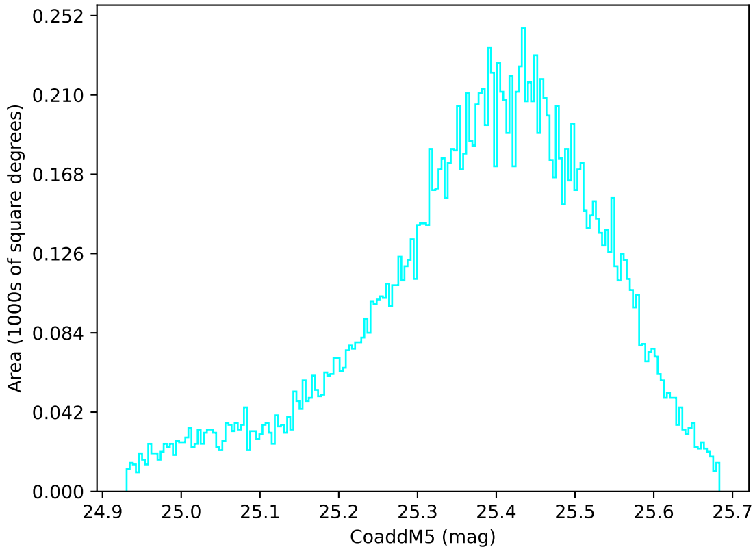
too_elab_r16_d2_gz_v3.4_10yrs WFD u band: CoaddM5
