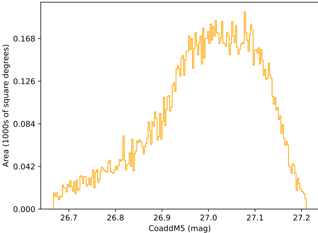
too_elab_r16_d2_gz_v3.4_10yrs WFD r band: CoaddM5
