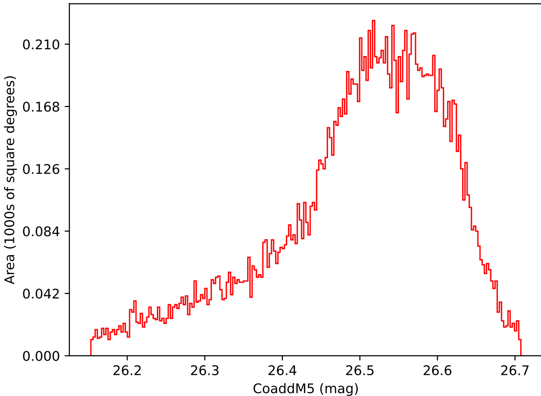
too_elab_r16_d2_gz_v3.4_10yrs WFD i band: CoaddM5
