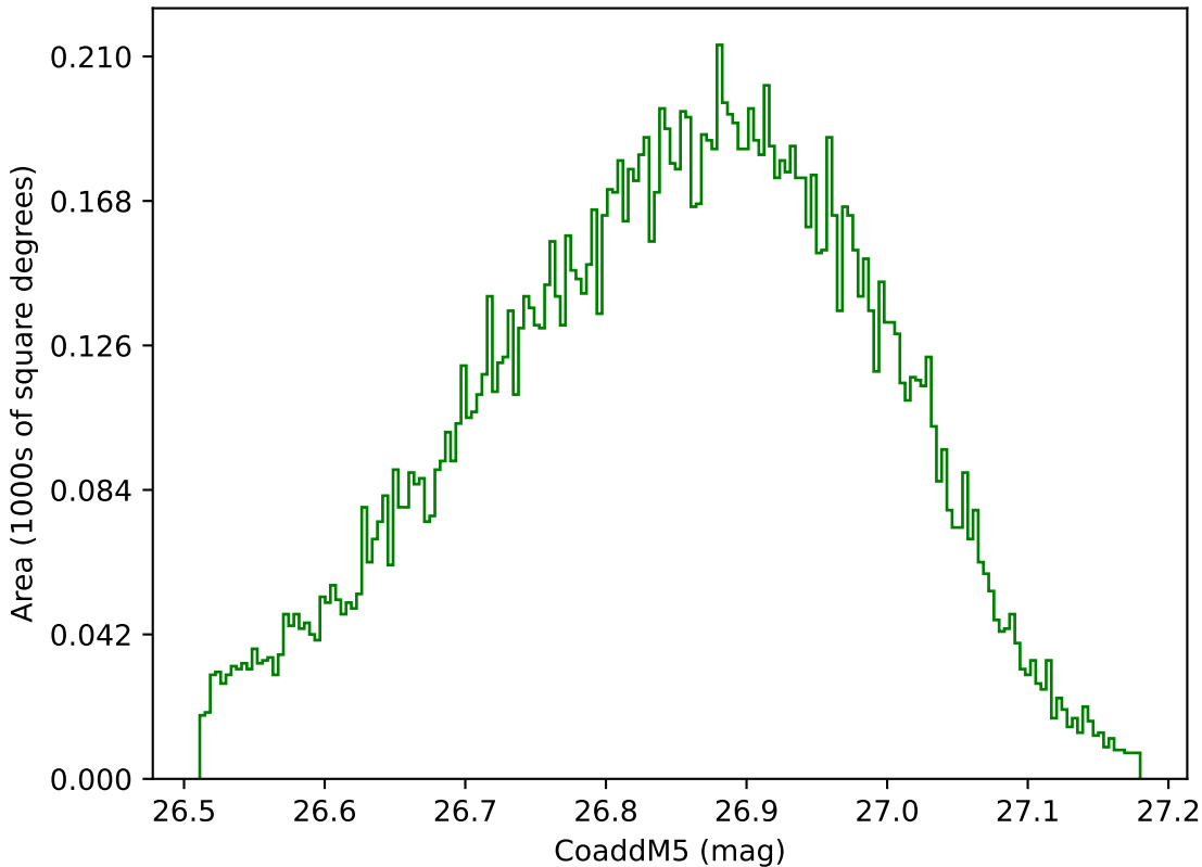
too_elab_r16_d2_gz_v3.4_10yrs WFD g band: CoaddM5
