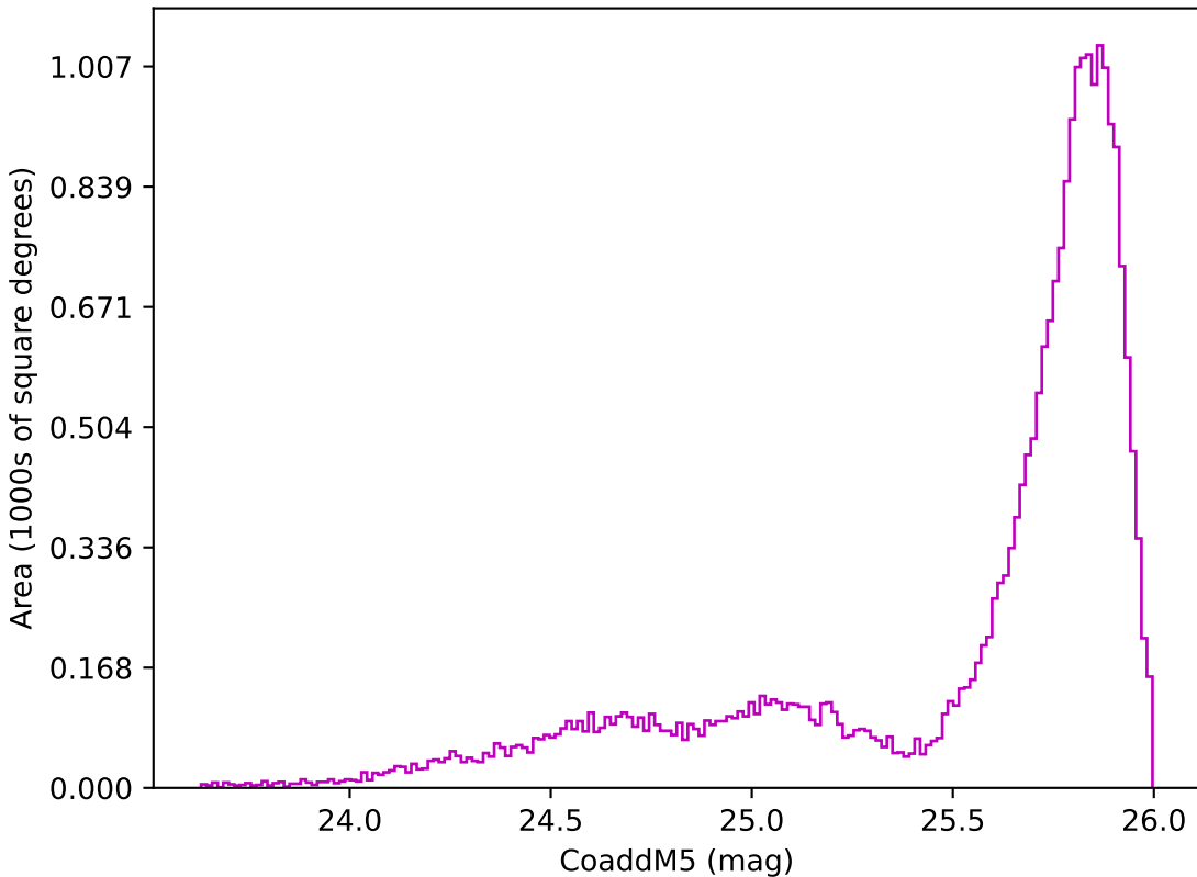
too_elab_r16_d2_gz_v3.4_10yrs All sky z band: CoaddM5
