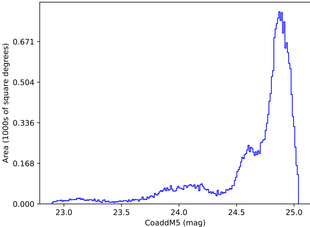
too_elab_r16_d2_gz_v3.4_10yrs All sky y band: CoaddM5
