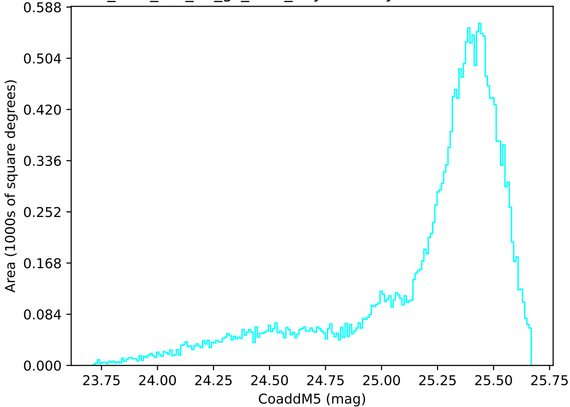
too_elab_r16_d2_gz_v3.4_10yrs All sky u band: CoaddM5
