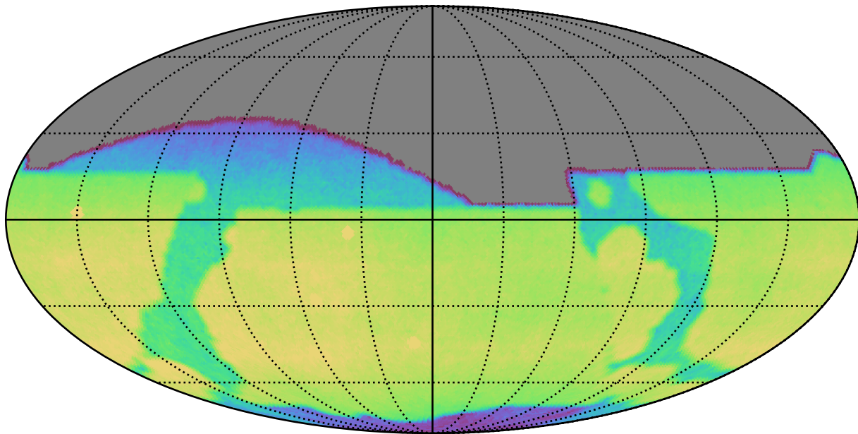
too_elab_r16_d2_gz_v3.4_10yrs All sky r band: CoaddM5
