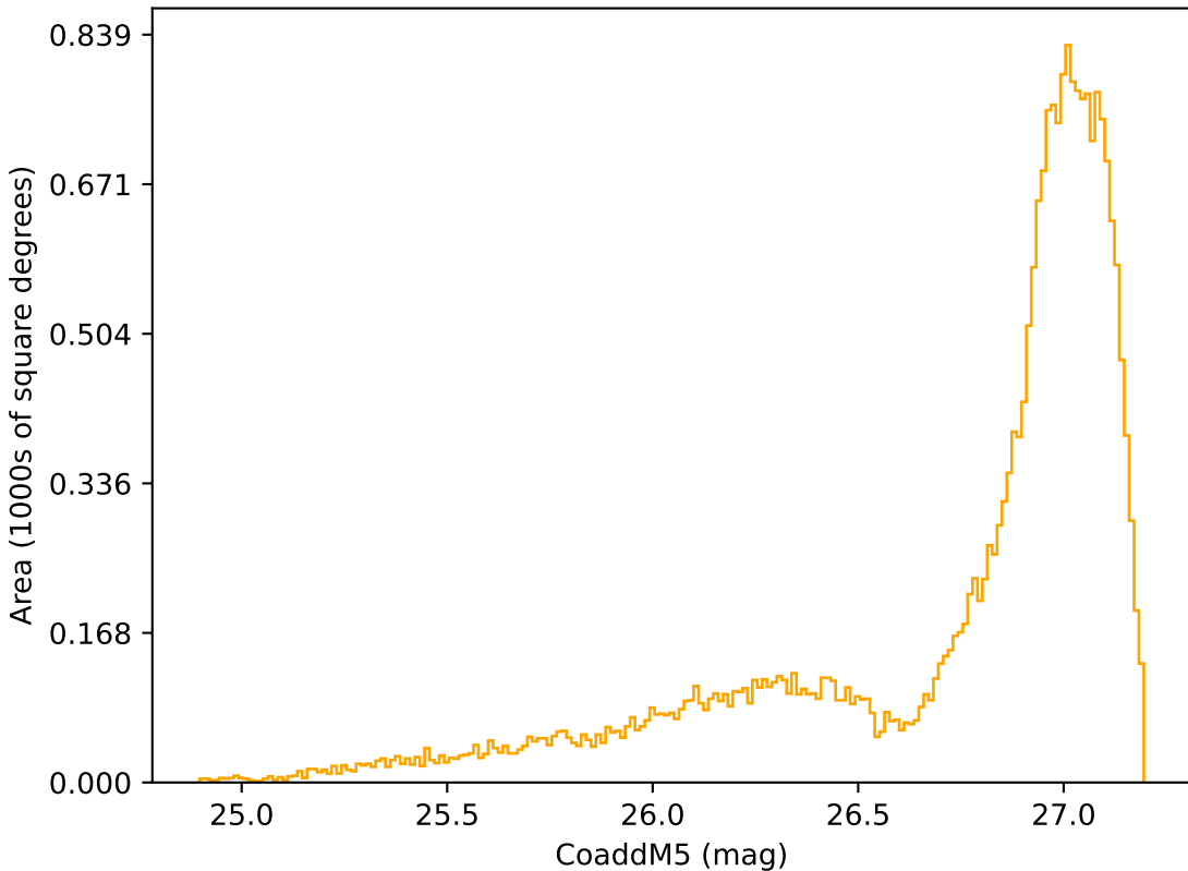
too_elab_r16_d2_gz_v3.4_10yrs All sky r band: CoaddM5
