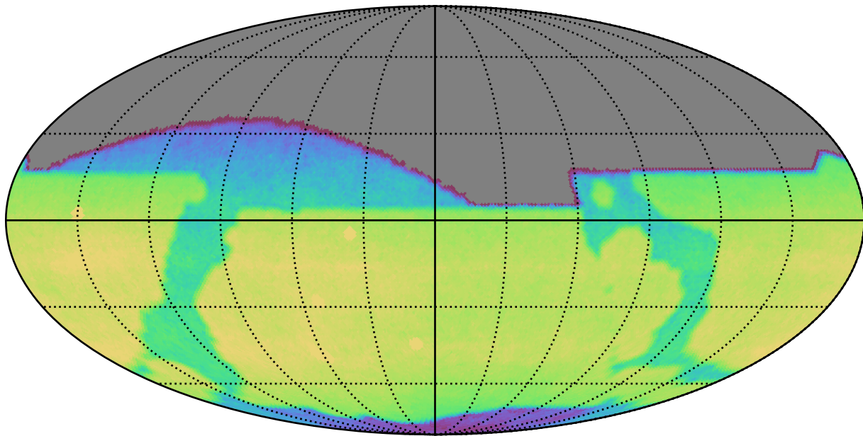
too_elab_r16_d2_gz_v3.4_10yrs All sky i band: CoaddM5
