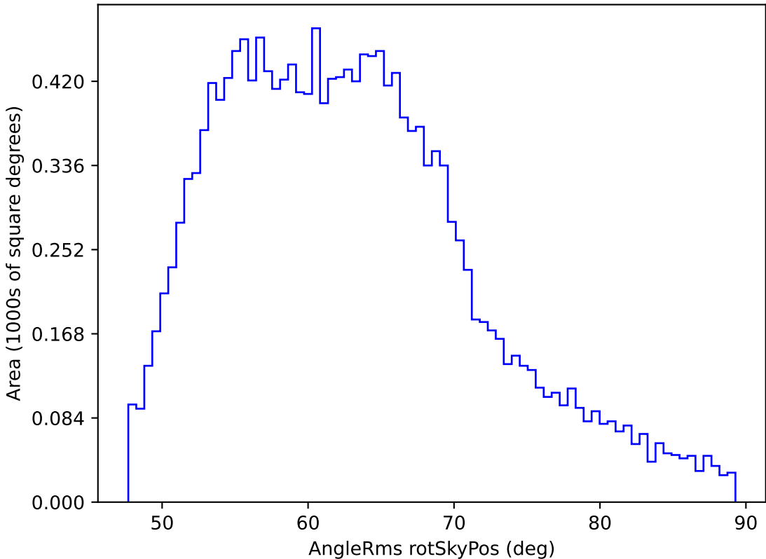
too_elab_r16_d2_gz_v3.4_10yrs WFD y band: AngleRms rotSkyPos
