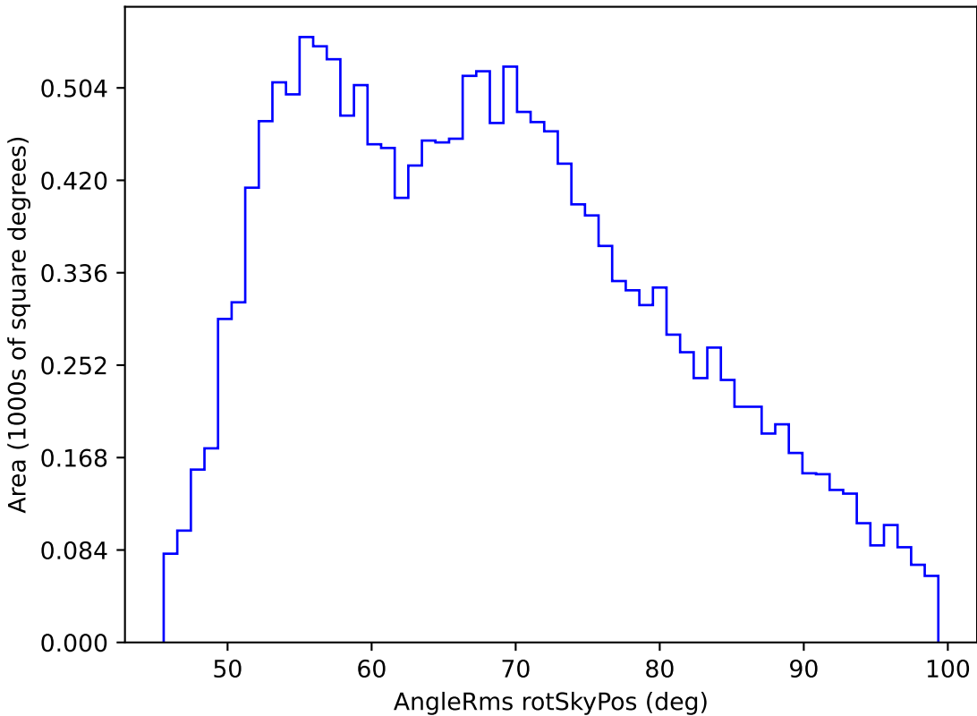
too_elab_r16_d2_gz_v3.4_10yrs WFD g band: AngleRms rotSkyPos
