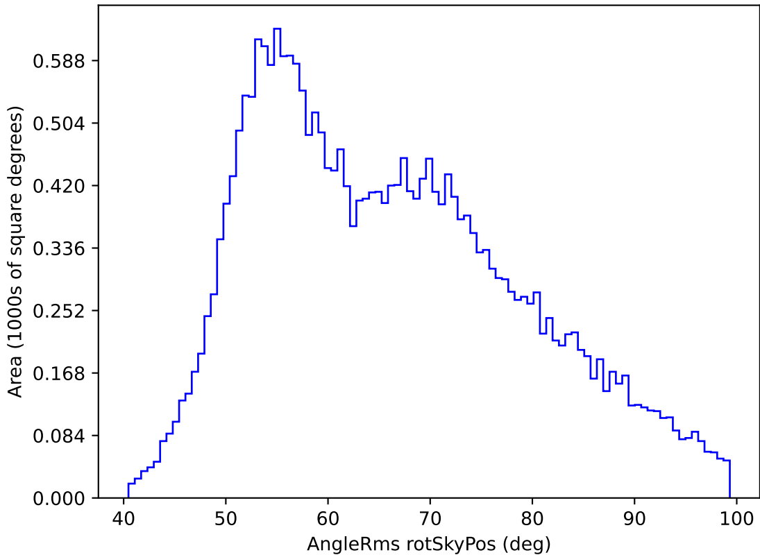
too_elab_r16_d2_gz_v3.4_10yrs All sky g band: AngleRms rotSkyPos
