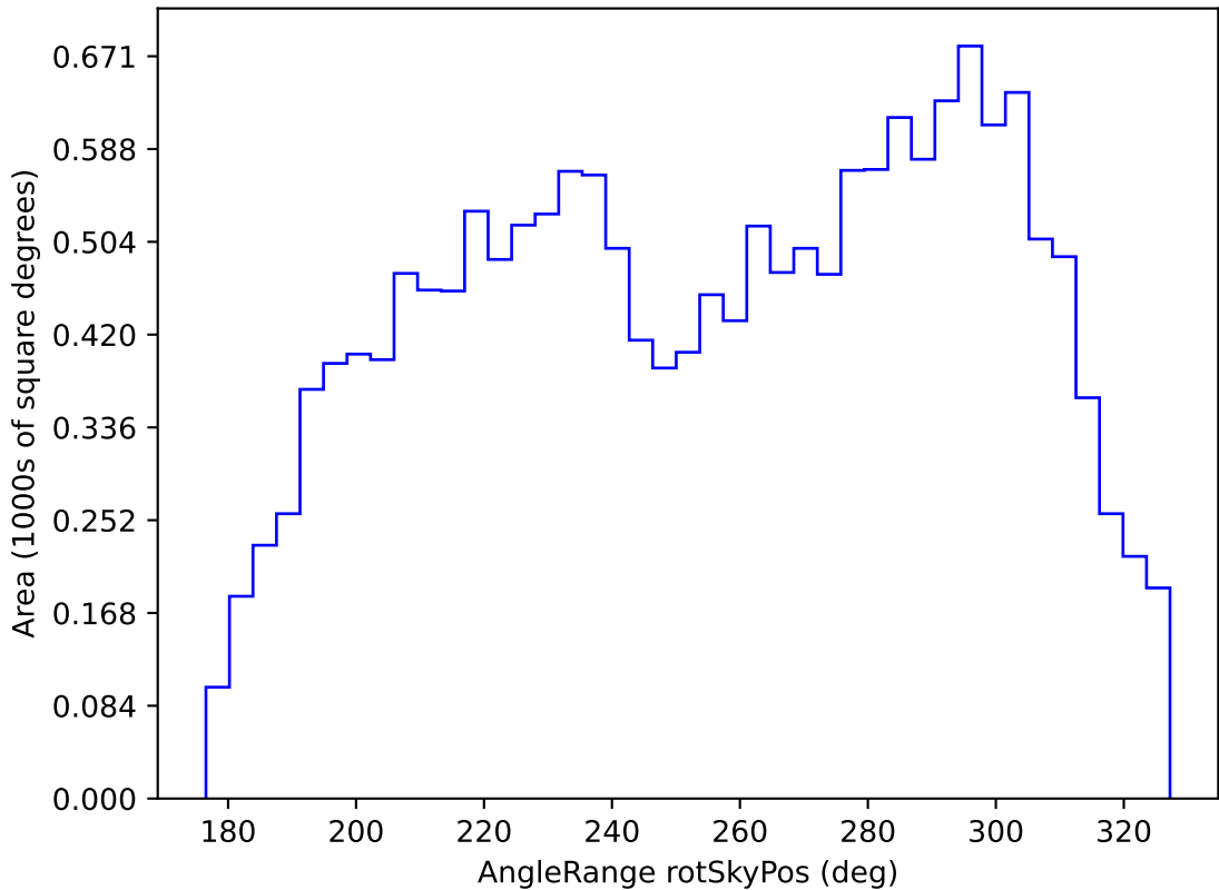
too_elab_r16_d2_gz_v3.4_10yrs WFD u band: AngleRange rotSkyPos
