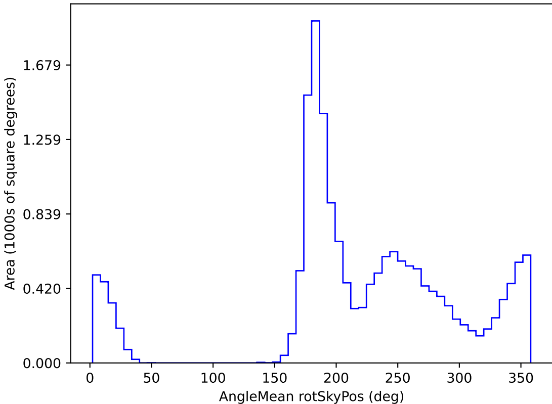
too_elab_r16_d2_gz_v3.4_10yrs WFD z band: AngleMean rotSkyPos
