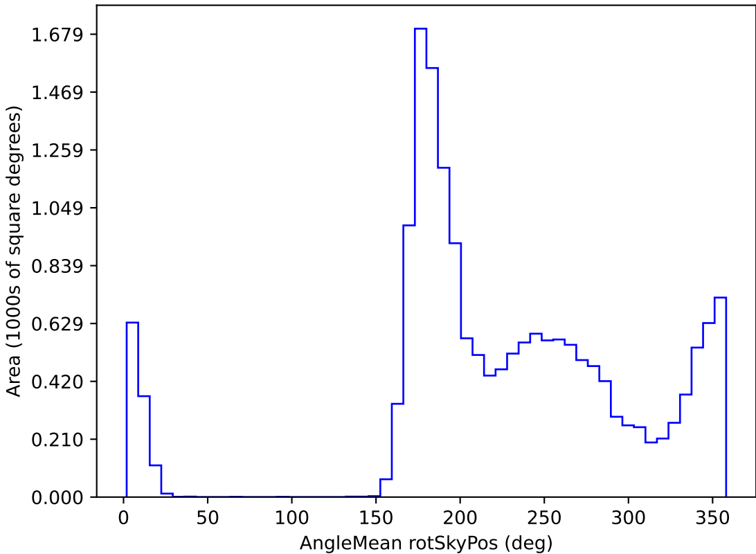
too_elab_r16_d2_gz_v3.4_10yrs WFD y band: AngleMean rotSkyPos
