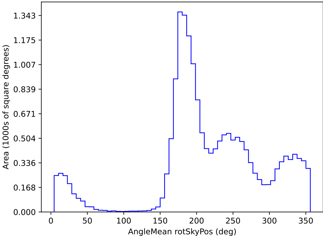
too_elab_r16_d2_gz_v3.4_10yrs WFD u band: AngleMean rotSkyPos
