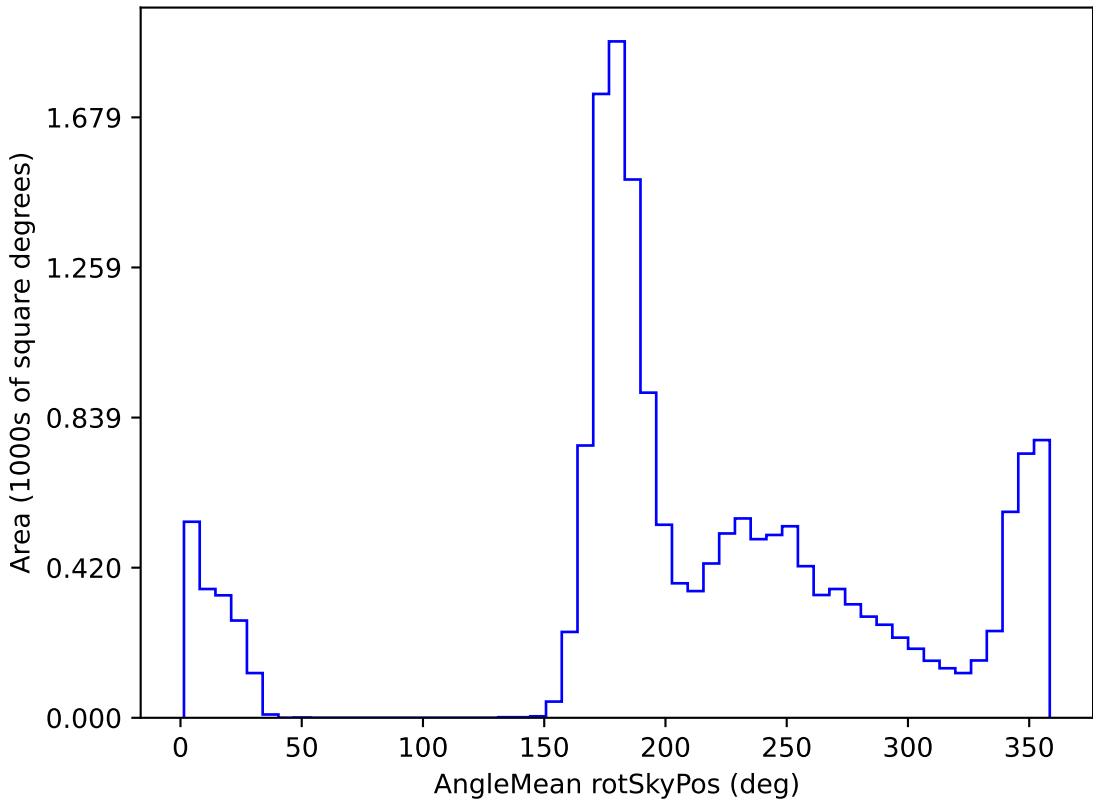
too_elab_r16_d2_gz_v3.4_10yrs WFD r band: AngleMean rotSkyPos
