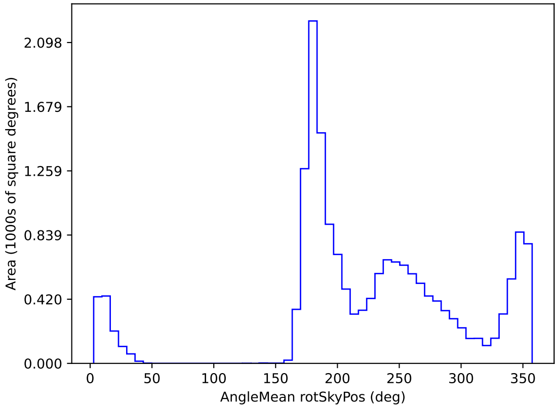
too_elab_r16_d2_gz_v3.4_10yrs WFD i band: AngleMean rotSkyPos
