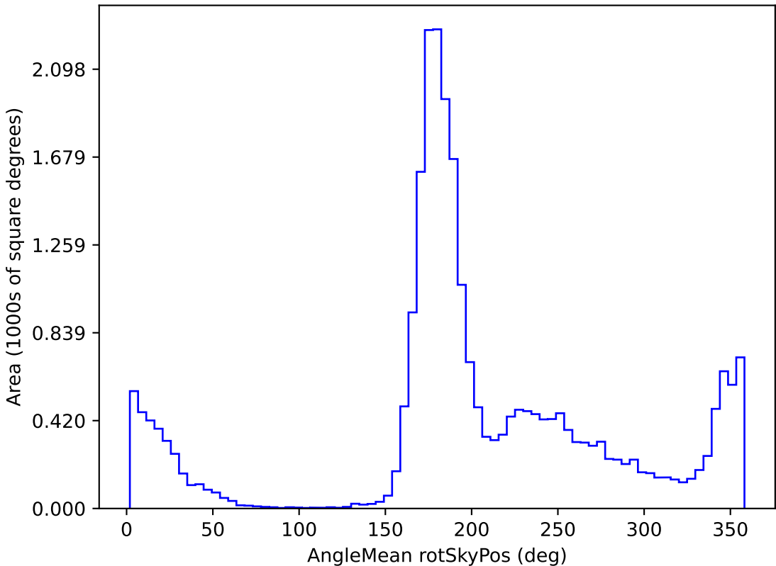
too_elab_r16_d2_gz_v3.4_10yrs All sky r band: AngleMean rotSkyPos
