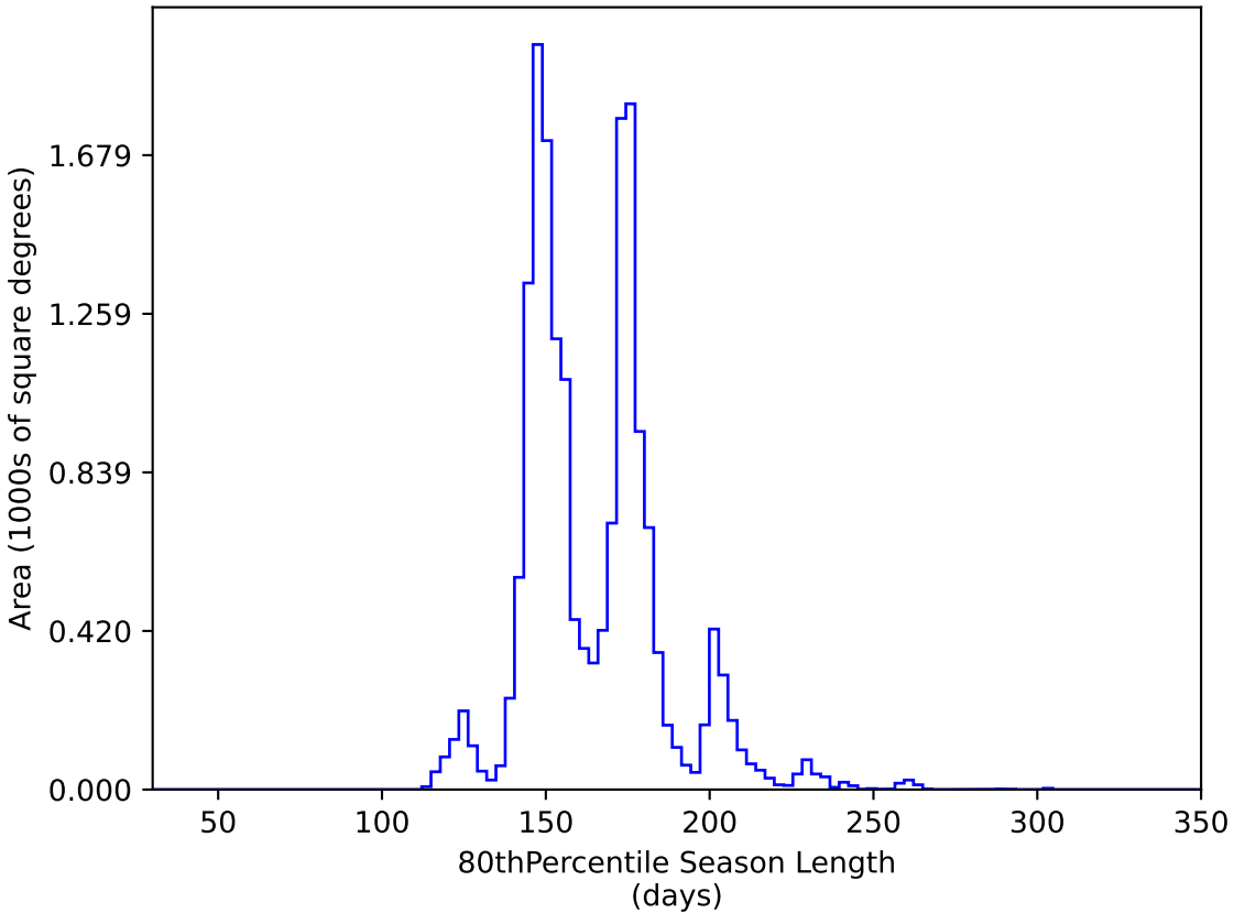
too_elab_r16_d2_gz_v3.4_10yrs WFD y band: 80thPercentile Season Length
