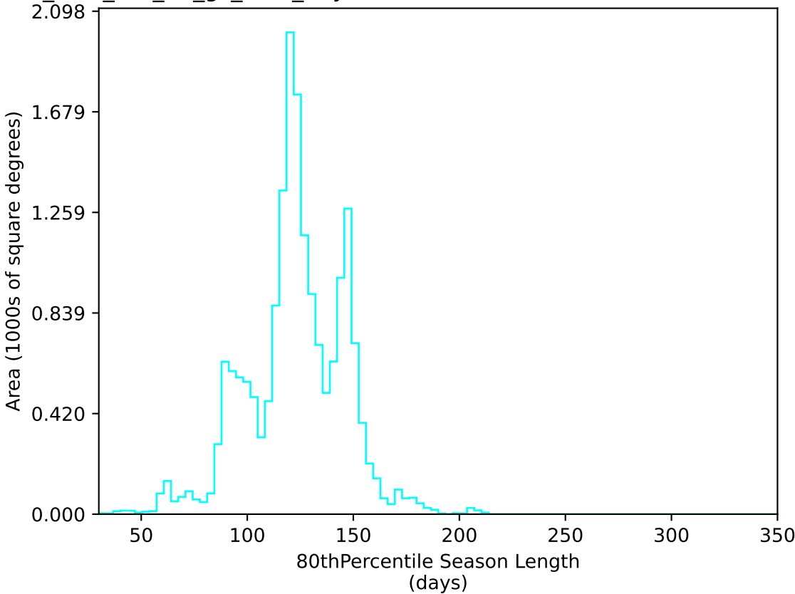
too_elab_r16_d2_gz_v3.4_10yrs WFD u band: 80thPercentile Season Length
