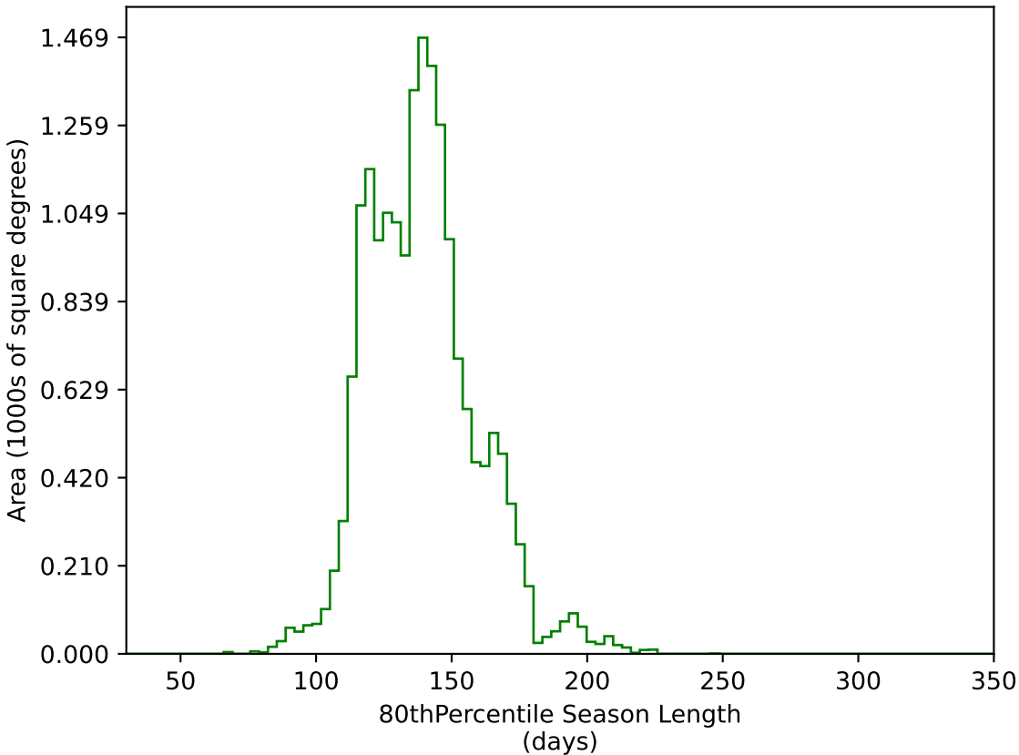
too_elab_r16_d2_gz_v3.4_10yrs WFD g band: 80thPercentile Season Length
