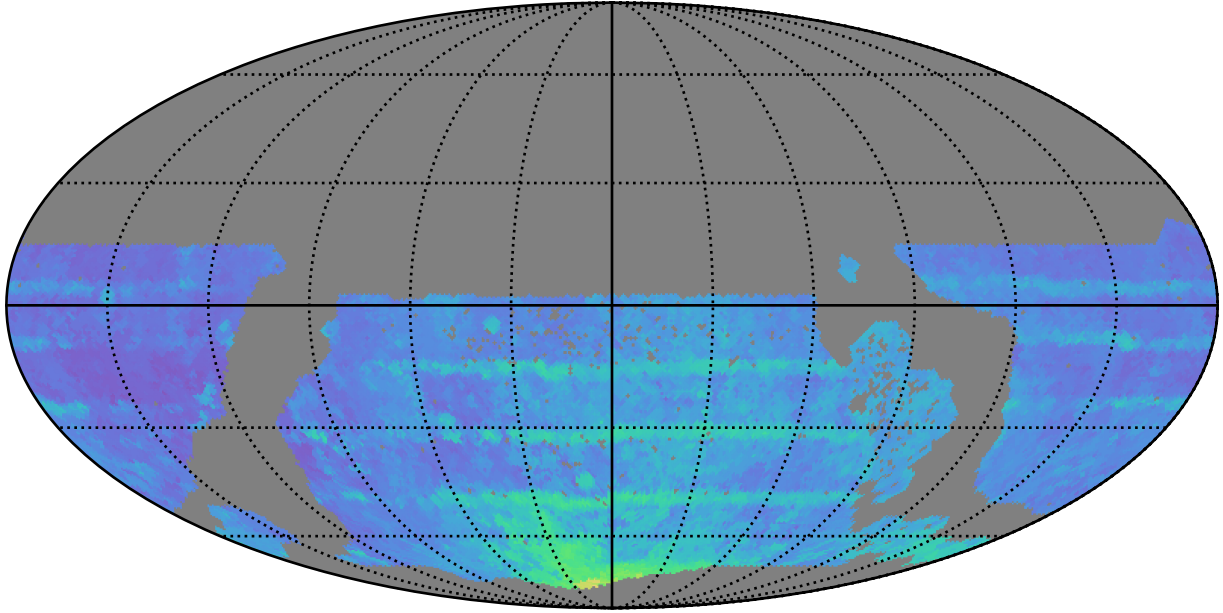
too_elab_r16_d2_gz_v3.4_10yrs WFD all bands: 80thPercentile Season Length
