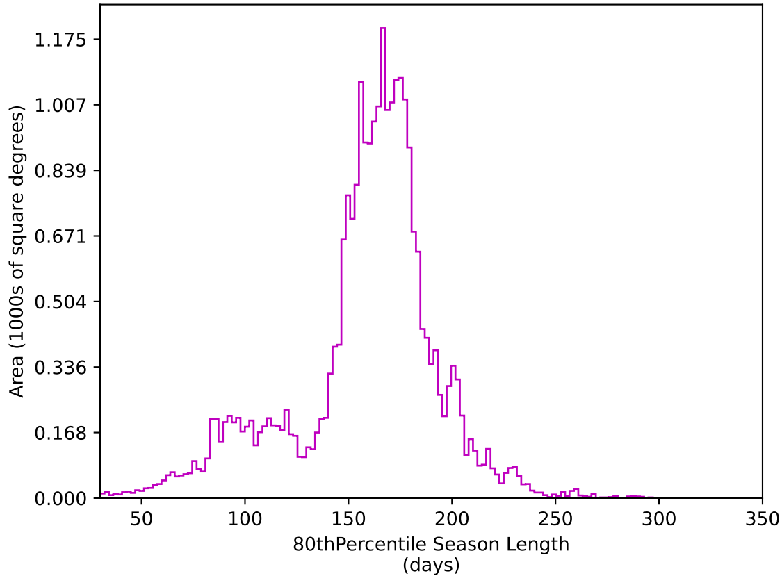
too_elab_r16_d2_gz_v3.4_10yrs All sky z band: 80thPercentile Season Length
