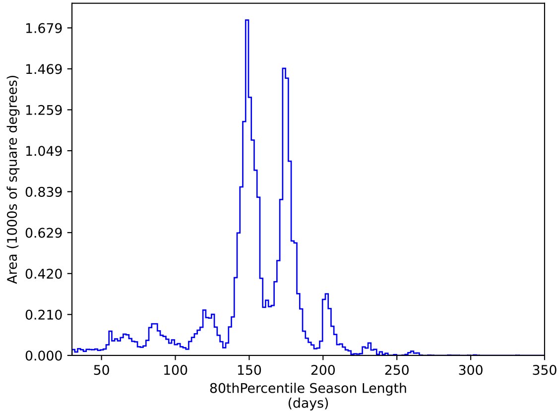
too_elab_r16_d2_gz_v3.4_10yrs All sky y band: 80thPercentile Season Length
