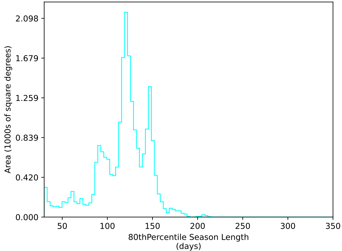
too_elab_r16_d2_gz_v3.4_10yrs All sky u band: 80thPercentile Season Length
