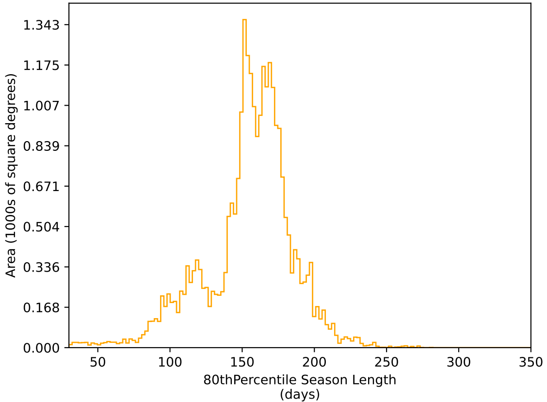
too_elab_r16_d2_gz_v3.4_10yrs All sky r band: 80thPercentile Season Length
