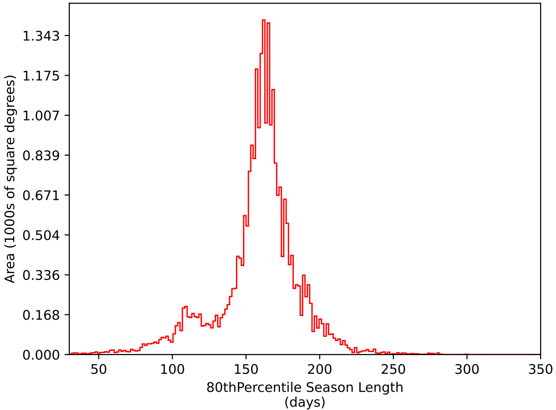
too_elab_r16_d2_gz_v3.4_10yrs All sky i band: 80thPercentile Season Length
