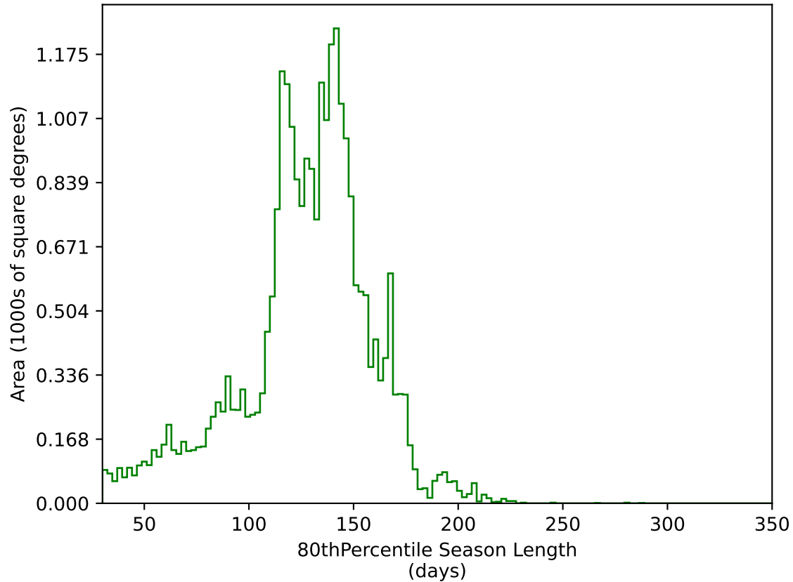
too_elab_r16_d2_gz_v3.4_10yrs All sky g band: 80thPercentile Season Length
