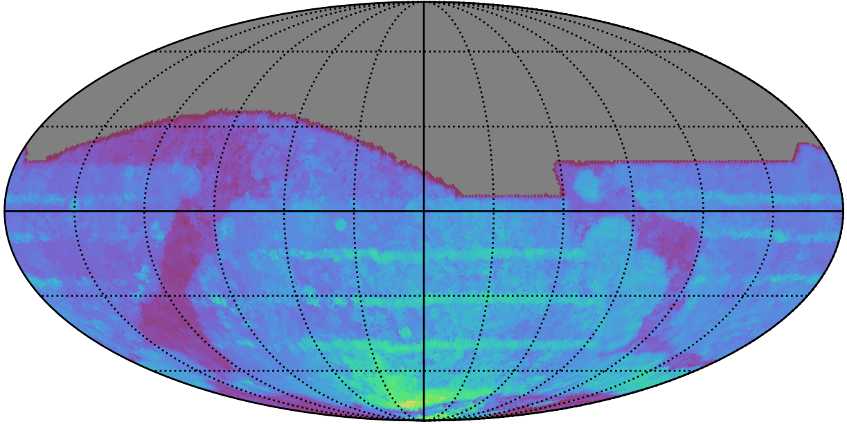
too_elab_r16_d2_gz_v3.4_10yrs All sky all bands: 80thPercentile Season Length
