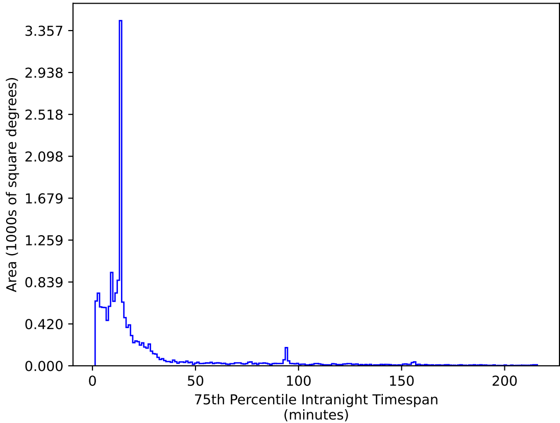
too_elab_r16_d2_gz_v3.4_10yrs WFD z band: 75th Percentile Intranight Timespan
