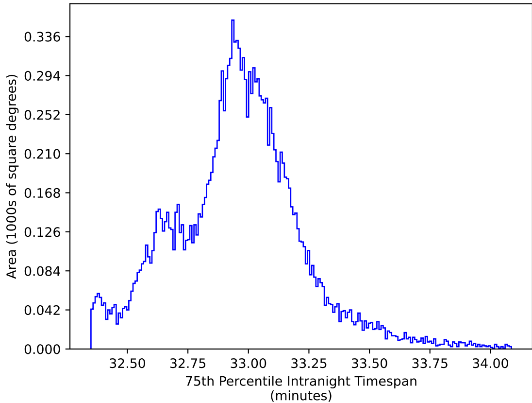
too_elab_r16_d2_gz_v3.4_10yrs WFD y band: 75th Percentile Intranight Timespan
