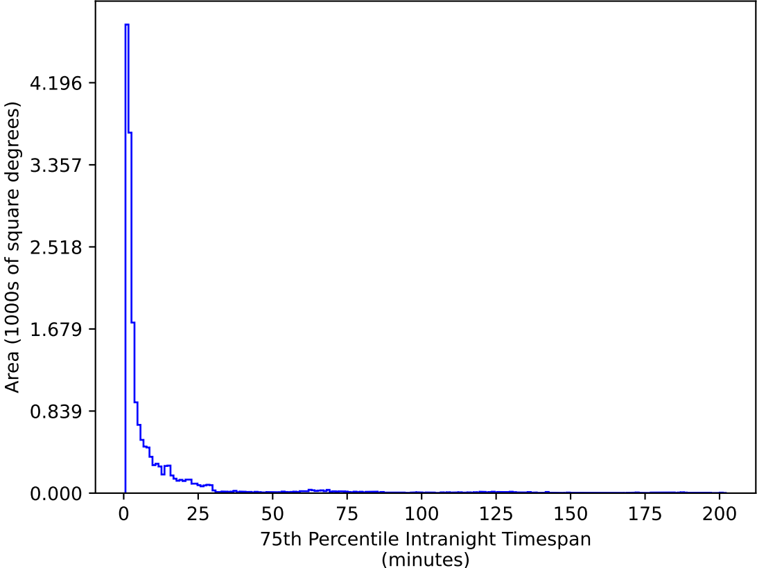
too_elab_r16_d2_gz_v3.4_10yrs WFD u band: 75th Percentile Intranight Timespan
