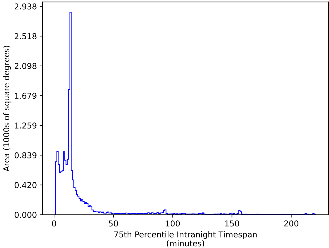
too_elab_r16_d2_gz_v3.4_10yrs WFD i band: 75th Percentile Intranight Timespan
