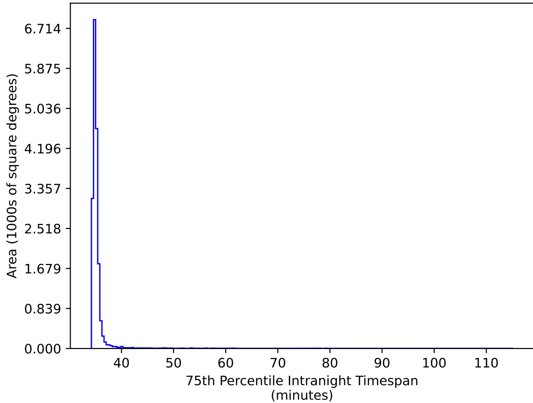
too_elab_r16_d2_gz_v3.4_10yrs WFD gr bands: 75th Percentile Intranight Timespan
