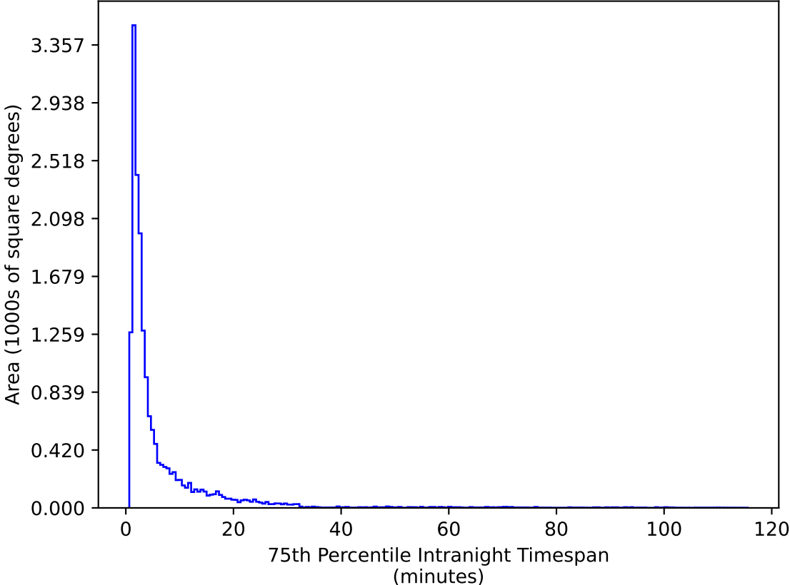
too_elab_r16_d2_gz_v3.4_10yrs WFD g band: 75th Percentile Intranight Timespan
