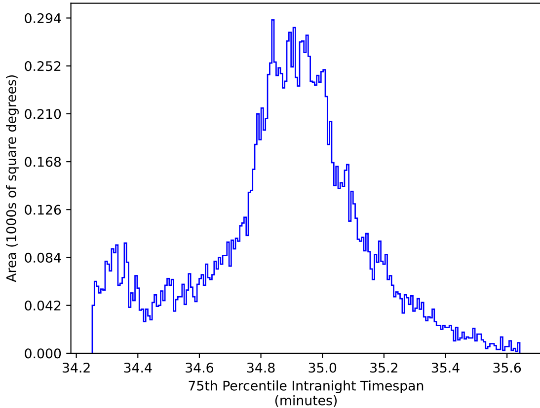
too_elab_r16_d2_gz_v3.4_10yrs WFD all bands: 75th Percentile Intranight Timespan
